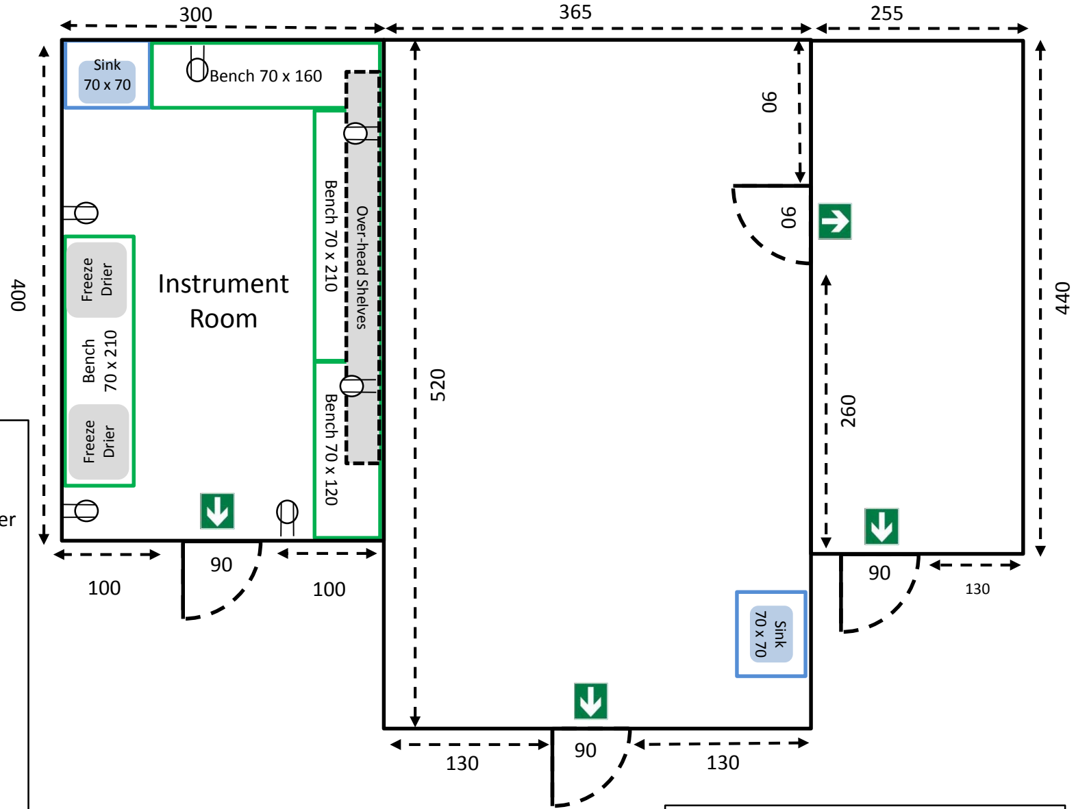
Green Houses I and II Abisko Scientific Research Station A-House Ground Floor
